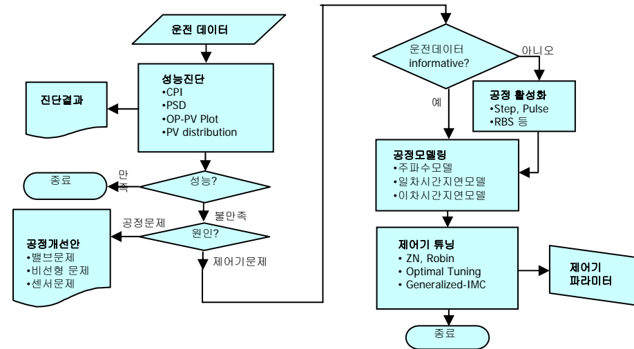
Loop Assessment Flow Sheet
